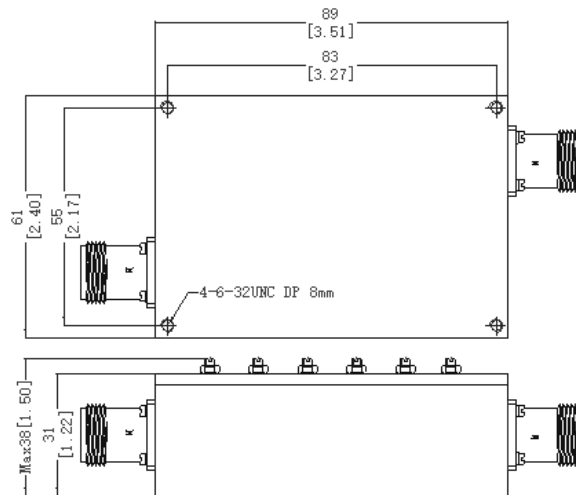
Physical Dimensions ( \pm 0.3\text{mm} )
